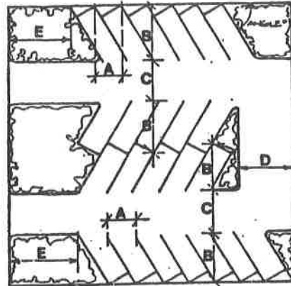
60° LAYOUT
