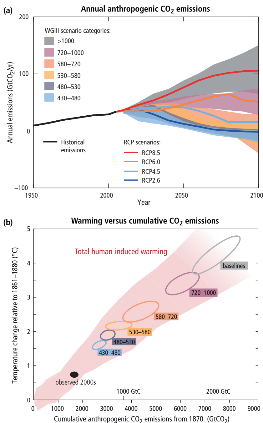
Figure SPM.5 | (a) Emissions of carbon dioxide (CO 2 ) alone in the Representative Concentration Pathways (RCPs) (lines) and the associated scenario categories used in WGIII (coloured areas show 5 to 95% range). The WGIII scenario categories summarize the wide range of emission scenarios published in the scientific literature and are defined on the basis of CO 2 -eq concentration levels (in ppm) in 2100. The time series of other greenhouse gas emissions are shown in Box 2.2, Figure 1. (b) Global mean surface temperature increase at the time global CO 2 emissions reach a given net cumulative total, plotted as a function of that total, from various lines of evidence. Coloured plume shows the spread of past and future projections from a hierarchy of climate-carbon cycle models driven by historical emissions and the four RCPs over all times out to 2100, and fades with the decreasing number of available models. Ellipses show total anthropogenic warming in 2100 versus cumulative CO 2 emissions from 1870 to 2100 from a simple climate model (median climate response) under the scenario categories used in WGIII. The width of the ellipses in terms of temperature is caused by the impact of different scenarios for non-CO 2 climate drivers. The filled black ellipse shows observed emissions to 2005 and observed temperatures in the decade 2000–2009 with associated uncertainties. [Box 2.2, Figure 1; Figure 2.3]
