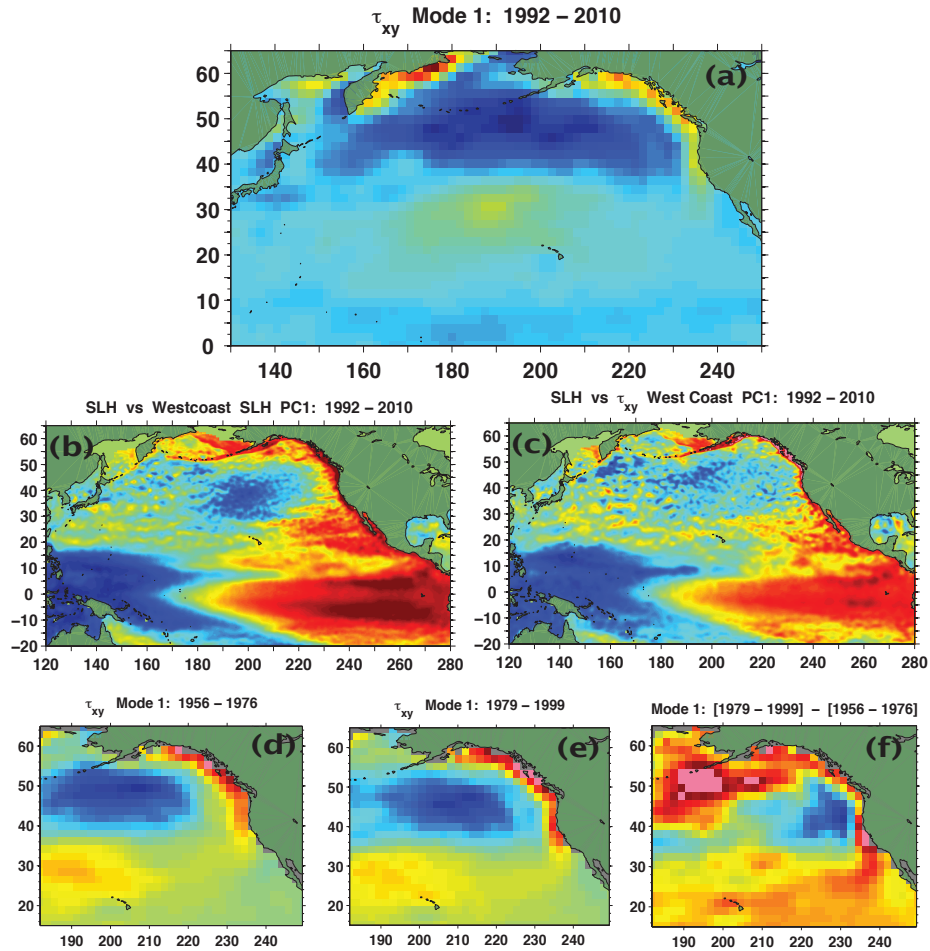
Figure 7. (a) Wind stress curl ( \tau_{xy} ) monthly anomaly mode 1 variability across the North Pacific basin. (middle) Correlation maps of altimetry SLH over the basin with mode 1 principal components over coastal region R1 (see Figure 2) of altimetry SLH (b) and \tau_{xy} (c). The range of r -values spans [-0.75, 0.75] in (b) and [-0.5, 0.5] in (c). (bottom) Wind stress curl monthly anomaly mode 1 patterns over the 1956-1976 (d) and 1979-1999 (e) epochs, with the difference between the two epochs (f) scaled to emphasize the change. Panels (d) and (e) have the same scaling as (a). Units are arbitrary.
