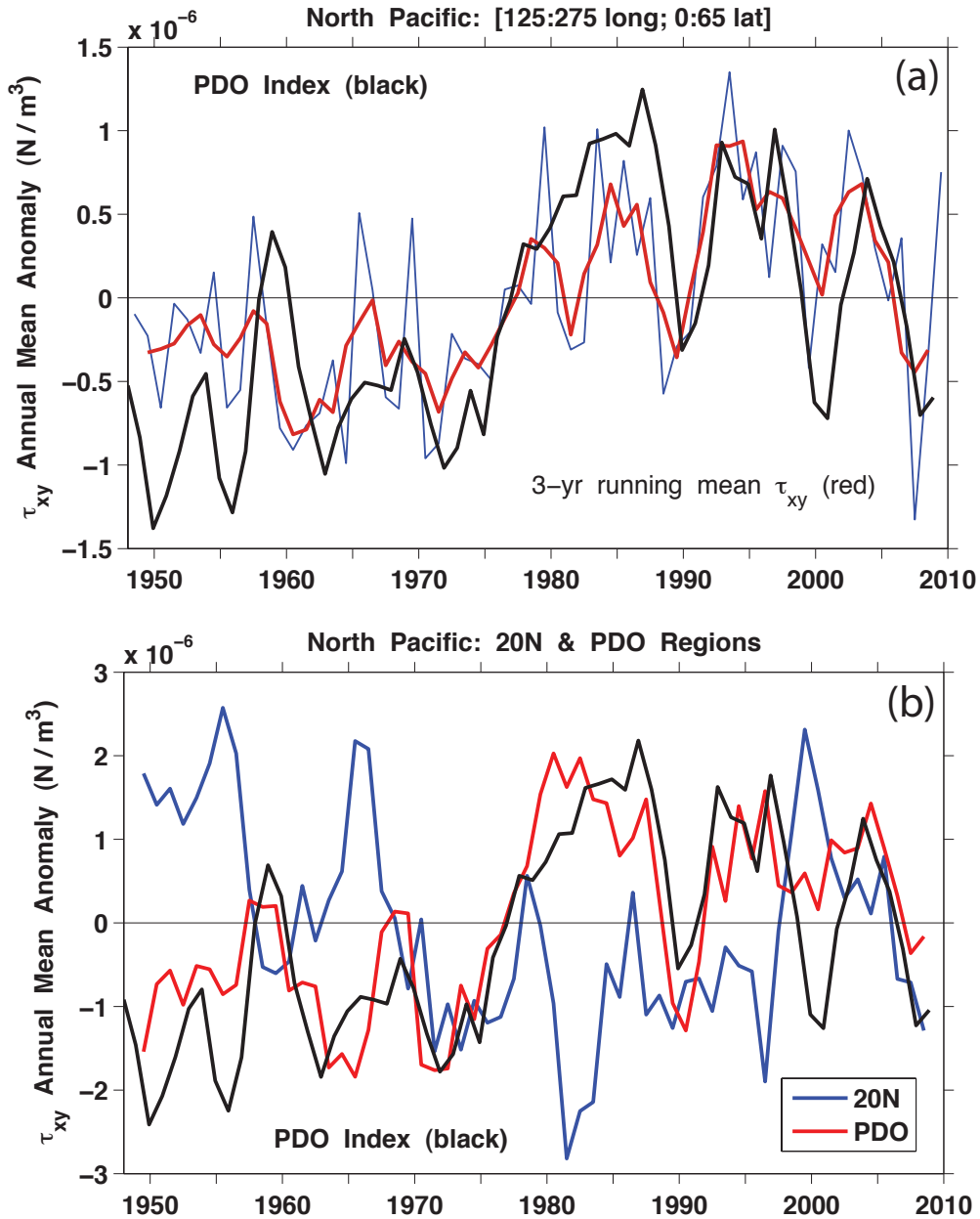
Figure 9. (a) Mean annual \tau_{xy} over the North Pacific north of the equator (thin blue) and 3-yr running means of \tau_{xy} (red) and the scaled PDO Index (black). Correlation of the 3-yr curves gives r = 0.76 , p < 0.001 . (b) 3-yr running means of mean annual \tau_{xy} over the entire North Pacific north of 20°N, i.e. excluding the tropics, (blue), and over the PDO region east of the date line (red), with the scaled PDO index (black).
