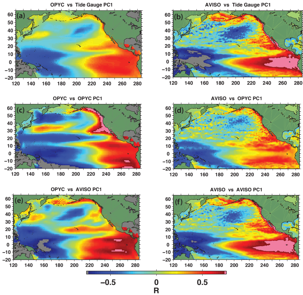
Figure 6. Correlation over 1992-2003 epoch between ocean model SLH anomalies over the entire North Pacific basin ( left panels ) and AVISO altimetry SLH anomalies ( right panels ) with EOF mode 1 principal components (PCs) of SLH anomalies of ( top ) coastal tide gauges, ( middle ) nearby ocean model, ( bottom ) coastal R1 altimetry. Note the generally weak correlation between eastern Pacific coastal sea level and Hawaii (202°E, 20°N).
