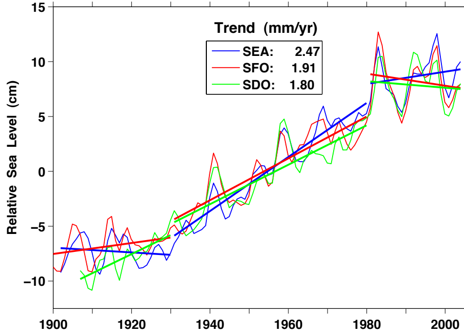
Figure 1. Decadal (lowpass-filtered) tide gauge SLH variability at the three stations with the longest records along the Pacific coast of North America at Seattle (SEA), San Francisco (SFO), and San Diego (SDO). The trends from 1930 to 1980 (box) are statistically significant from zero at the 97.5% level, while of the others, only the trend at SDO prior to 1930 is.
