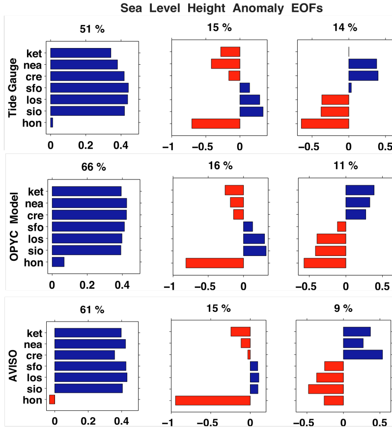
Figure 5. ( top ) EOF's of the first three modes of inverse barometer-corrected tide gauge SLH anomalies for 1948-2003 at stations (see Figure 2a for locations) KET (Ketchikan, AK), NEA (Neah Bay, WA), CRE (Crescent City, CA), SFO (San Francisco, CA), LOS (Los Angeles, CA), SIO (La Jolla, CA), and HON (Honolulu, HI). The observed patterns of variability are comparable to Chelton and Davis (1982), but here with longer records. The variance explained by each mode is indicated. ( middle ) OPYC model EOFs obtained for SLH anomalies over the 1948-2003 epoch at grid points approximately 1^\circ west of the tide gauge station observations. ( bottom ) AVISO satellite altimetry EOF's obtained at grid points near those for the OPYC model over the 1992-2009 epoch. Note the strong similarity of the spatial patterns between the tide gauge, OPYC model, and satellite observations.
