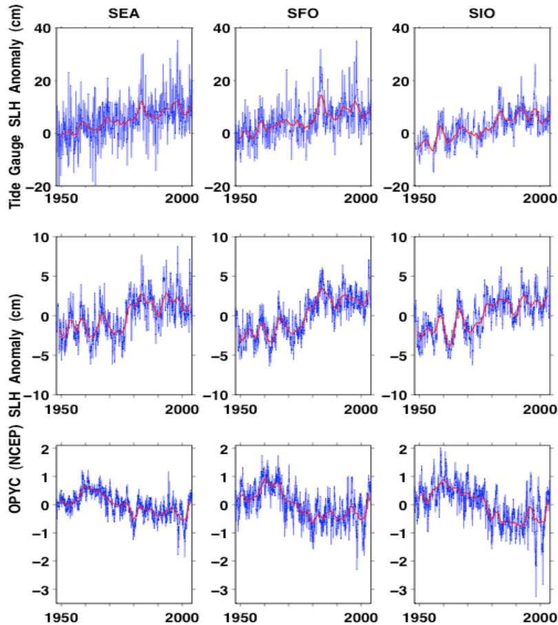
Figure 4. ( top ) Observed tide-gauge sea level (sea level pressure-corrected) monthly anomalies (long-term mean removed), with 3-yr running means (red lines) in all panels. The San Francisco (SFO) and La Jolla (SIO) regions are thought to be tectonically vertically stable, while the Seattle (SEA) region is probably not. ( middle ) Model sea level height twice-monthly anomalies from the OPYC model hindcast forced with NCEP Reanalysis wind stress and heat flux anomalies. Note that the trends are weaker than the observed ( top, different scales ). ( bottom ) Model sea level height twice-monthly anomalies from the OPYC ocean model hindcast forced only with NCEP heat flux anomalies. Note that the anomalies in this simulation are generally much smaller than forcing with both wind stresses and heat fluxes, indicating the dominance of wind-stress forcing of RSL fluctuations.
