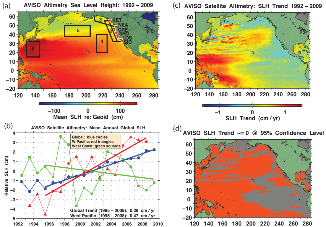
Figure 2. (a) Mean SLH across the North Pacific basin from 1992-2009, with locations of tide gauge stations used to determine coastal-to-basin-wide spatial relationships indicated. (b) Mean annual RSL curves across regions along the U.S. Pacific coast (region 1, green; region 2, dashed green) and in the Western Pacific (region 6, red), compared with global MSL (blue). Regions 1-6 are referred to as R1-R6 in the text. Western Pacific and global upward trends in (b) are statistically significant from zero at the 97.5 level, while the West Coast trend is not. (c) Least squares trends in SLH across the North Pacific basin, with (d) the T-test trend analysis showing regions where the trend is significantly different from zero at the 95% level (red).
