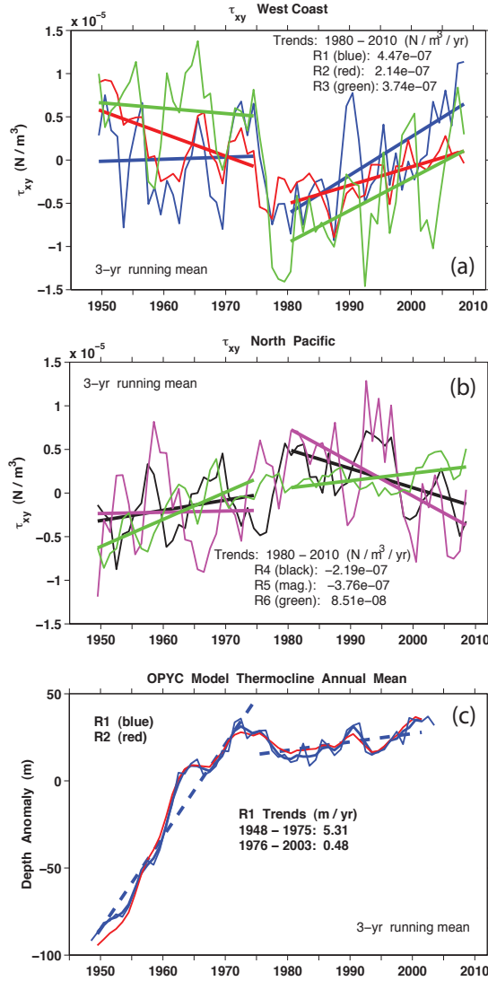
Figure 8. Mean wind stress curl, \tau_{xy} , 3-yr running means over (a) the eastern Pacific boundary regions R1, R2, & R3 (see Figure 2) and (b) non-coastal regions R4, R5, and R6. All trends after the mid-1970's regime shift are significant at the 97.5% confidence level or higher, while only those for R2 in (a), R6 in (b), are. (c) Thermocline depth anomaly (thin blue) 3-yr running mean estimates (thick blue, red) from the OPYC model simulation forced with NCEP wind stress and heat flux anomalies over coastal regions R1 and R2. These model thermocline depth variability estimates were obtained by calculating the depth of the third isopycnal layer, which did not shoal, and correcting for the climatology at each grid point before obtaining the annual averages over each region. Trends (dashed lines, significant at the 97.5% level) show the dramatic change after the mid-1970's regime shift.
