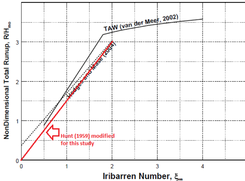
Figure 17 - Non-dimensional Total Runup vs. Iribarren Number
